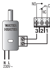
Connection to a water heater
